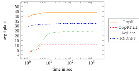
Figure 1: Average number of plans generated over time.
