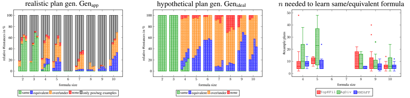
Figure 3: Relative number of instances where the same, an equivalent formula, an over/under-approximation, or no related formula at all is found. Order of plan-generation approaches for each formula size: TopK, TopKFill, AgDiv, RNDhFF. Rightmost plot: distribution of number of plans needed, in Gen ideal setup, to solve an instance, for those instances commonly solved by TopKFill, RNDhFF, and AgDiv.
